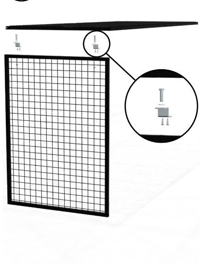
07 ROOF CONNECTION KIT
