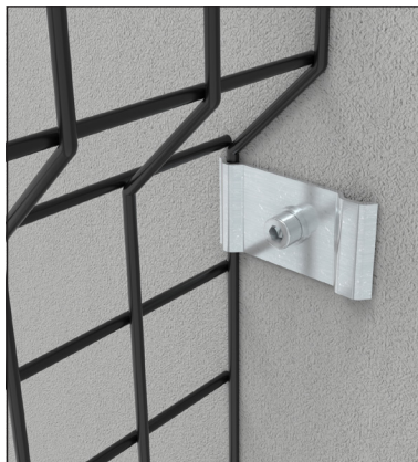
05 MODULA MESH TO WALL CONNECTION KIT
