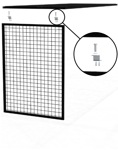
07 ROOF CONNECTION KIT
