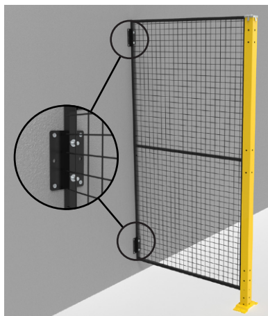
08 PANEL TO WALL CONNECTION KIT
